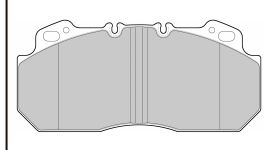
FCV1813B (250x114x28mm) 29090
