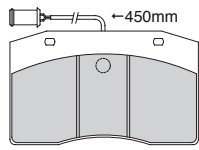
FCV1614 (180x106x20mm) 29186
