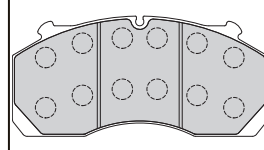
FCV1821B (249x117.5x30mm) 29150
