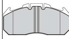
DCV1404BFE (250x118x30mm) 29156
