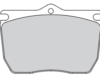
FCV898 (162x111x28mm) 29016
