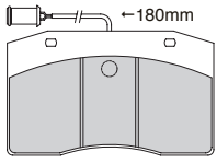
DCV801 (180x106x20mm) 29075
