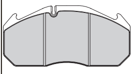
DCV1584B (250x118x30mm) 29053
