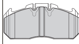
DCV1653BFE (250x118x30mm) 29156
