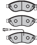
FD7427A TRW 24922 103.8 x 56.1 x 17.2mm
