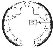
N1502 LKD 254 x 89 x 5.8mm
