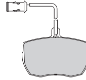
FD6490V BRE 29038 110 x 73 x 18.3mm
