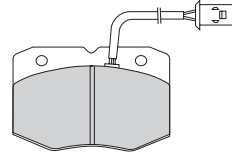
FD6806V BRE 29140 110 x 73 x 18.3mm
