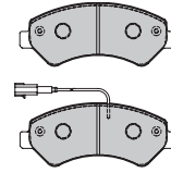
FD7269V BRE 24466 169.3 x 69.2 x 19mm
