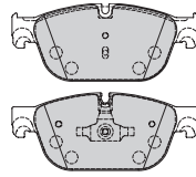
FD7485A ATE 25069 180.1 x 75.1 x 16.9mm
