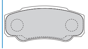
FD7270V BOS 24465 136.9 x 48.8 x 18.8mm
