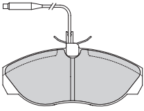
FD6889V LUC 21797 145 x 61 x 18.9mm
