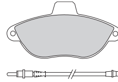
FD6896V BRE 23919 165 x 69.3 x 19.1mm
