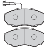
FD7268V BRE 24466 169.3 x 69.2 x 19mm
