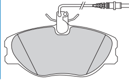
FD6895V BRE 23917 141 x 65.9 x 19.1mm
