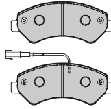
FD7485A ATE 25069 180.1 x 75.1 x 16.9mm
