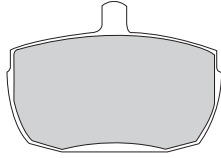
FD6261V LKD 20653 102 x 75 x 18mm
