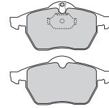
FD7411A MAN 24415/24416/24417 131.5 x 59.6 x 18.2mm
