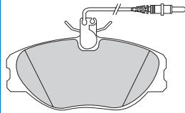
FD6895V BRE 23917 141 x 65.9 x 19.1mm
