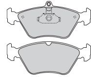
FD7025A ATE 21829 156/155 x 74 x 19.6mm
